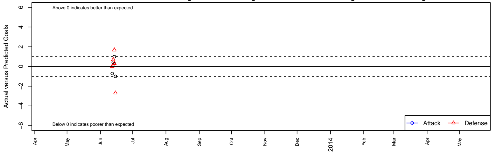
Colorado United White B95 Dots are actual minus expected GF (blue circles) and GA (red triangles). Blue line is smoothed change in attack strength. Red is smoothed change in defense strength.
